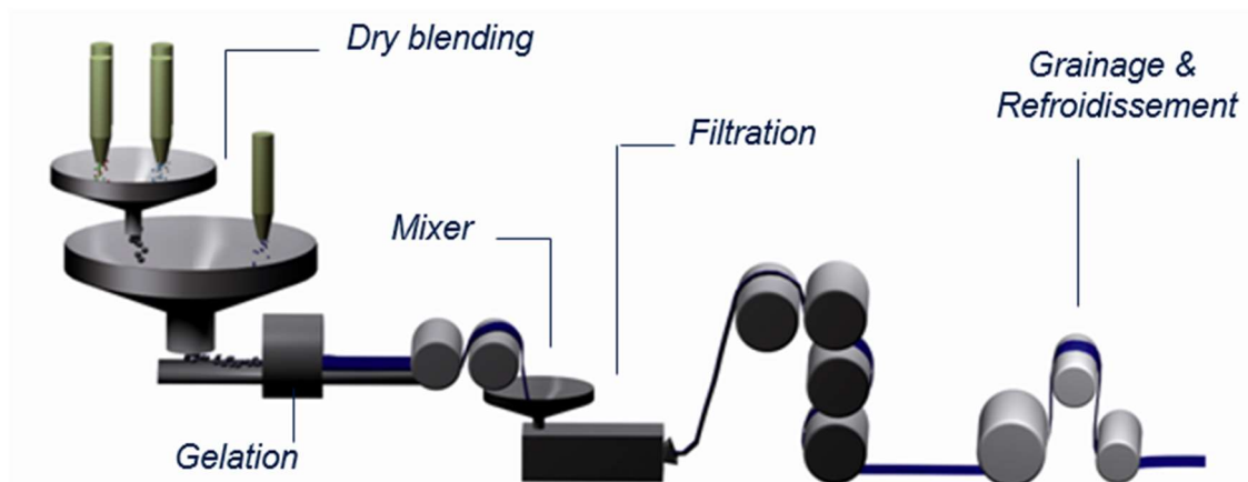
Figure 1 : Process de Calandrage
